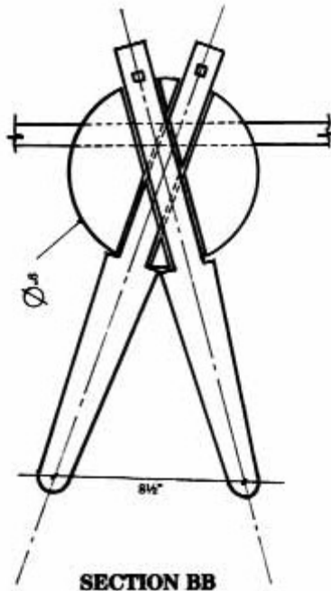
SECTION BB
